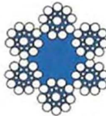
6 x 19S+FC
